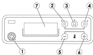
Fig. 6 - Control panel
