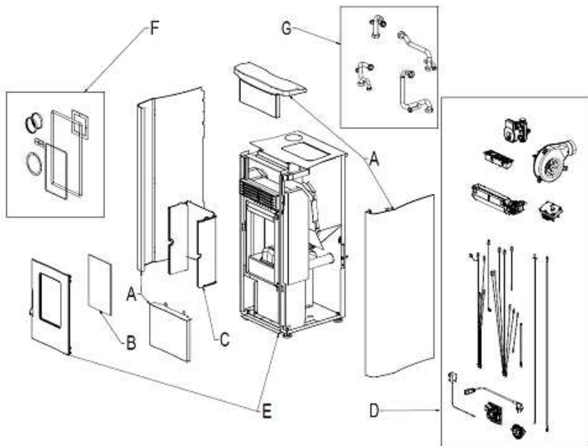
Fig. 1 - Exploded drawing
