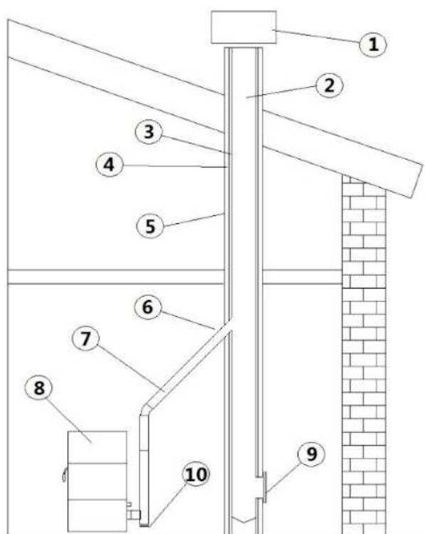
Fig. 2 - Chimney components
