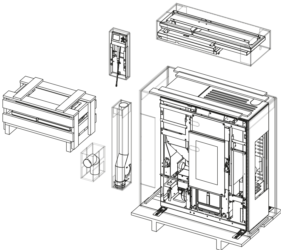
PACKAGING STOVE+CLADDINGS+ACCESSORIES
