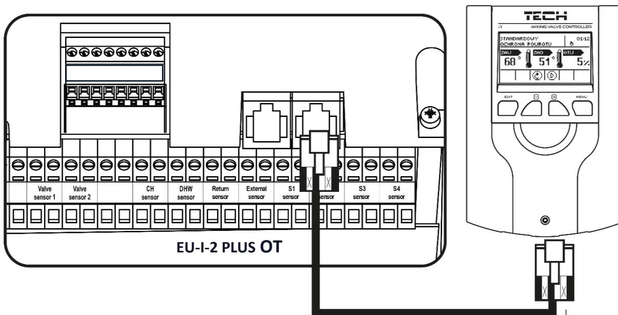
Example connection between additional valve and EU-i-2 Plus OT main controller
